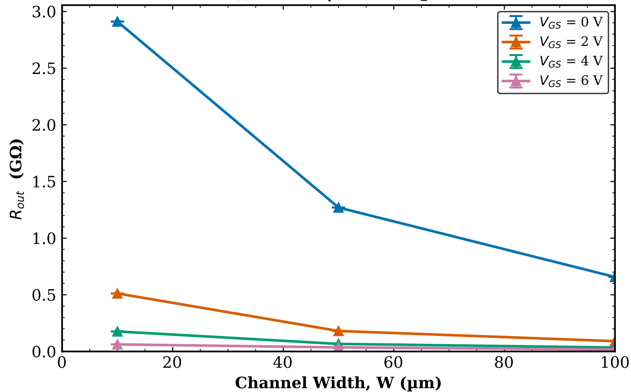
TFT1 Transistor 2 R_{out} vs W | L = 80\text{ }\mu\text{m}
